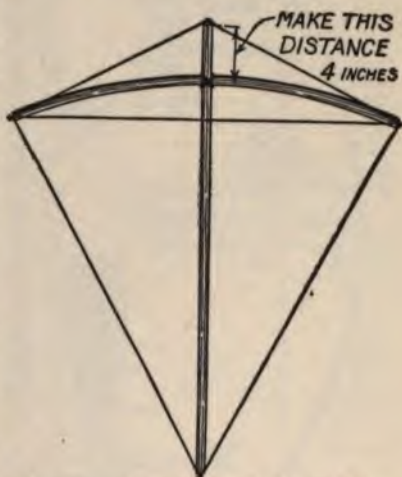
FIG. 19. — Framework of Malay Kite.
